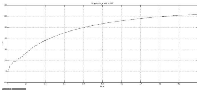
Fig 11. Output voltage of solar panel with MPPT
