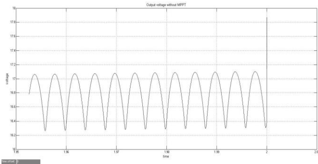
Fig 10. Output voltage of solar panel without MPPT
