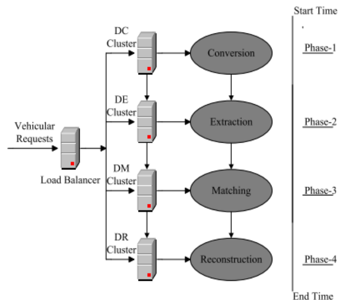
Fig.3 Task Level parallel Processing Procedure from [1]
