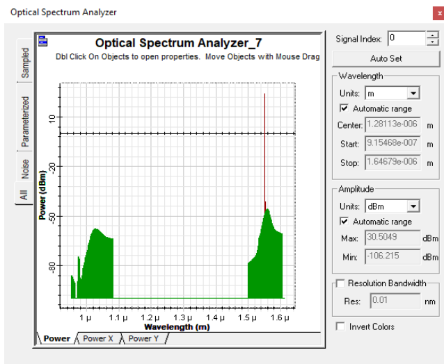
Fig. 5. OSA output of EDFA2 with p_p=150\text{mw} and L=5\text{m}
