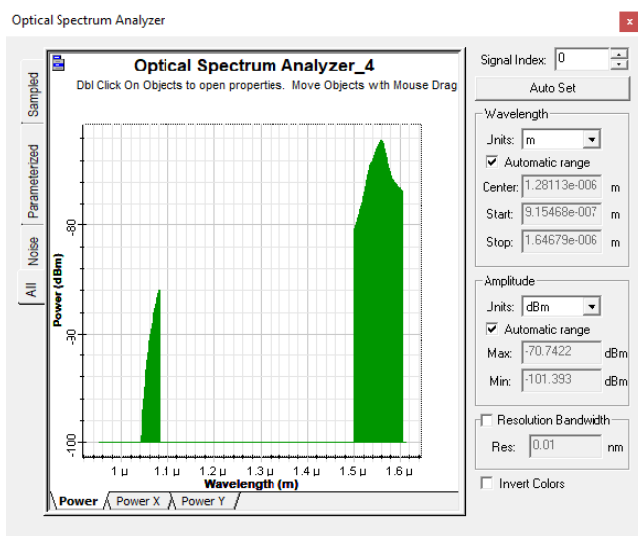
Fig. 6. OSA backward output of EYCDFA with p_p=100\text{mw} and L=10\text{m}
