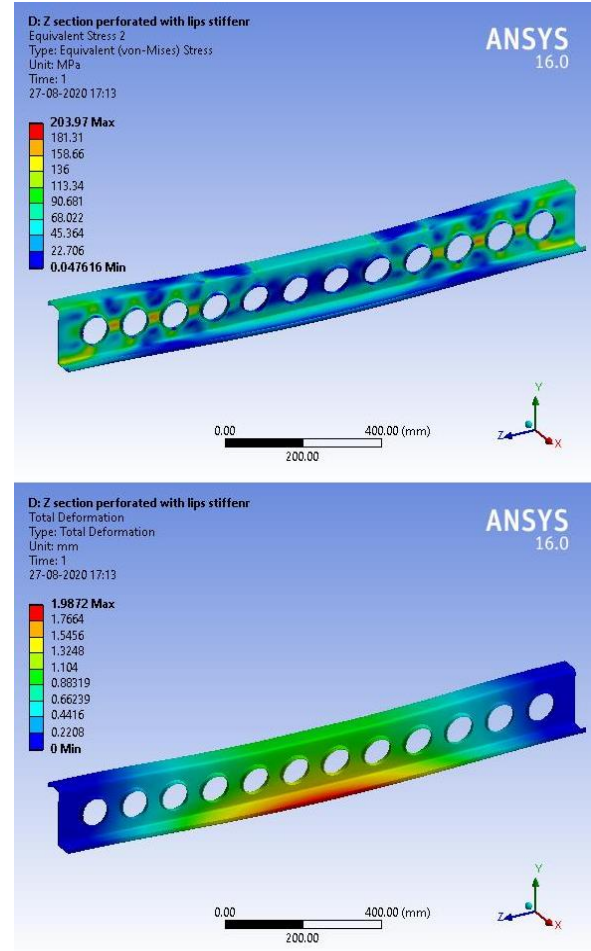
Fig. 9 Deformed shape of ZLPS1500
