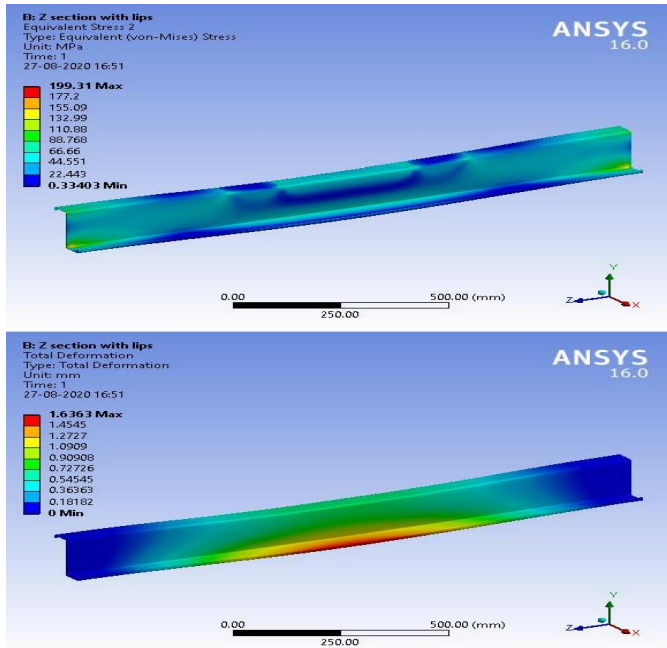
Fig. 7 Deformed shape of ZL1500
