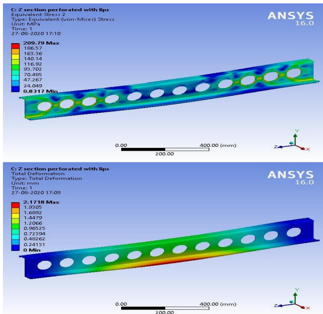
Fig. 8 Deformed shape of ZLP1500
