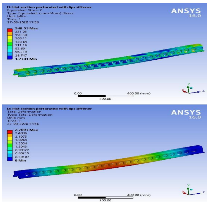
Fig. 13 Deformed shape of HLPS1500
