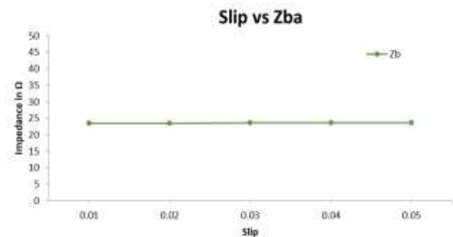
Fig.11. Slip vs Reverse branch impedance
