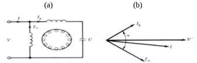
Fig. 1. (a) PSCRSPIM Circuit (b) Vector Diagram
