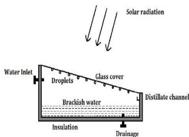
Fig. 1. Schematic diagram of a conventional solar still
