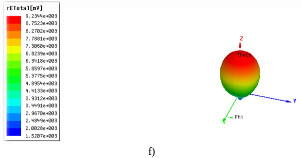
Fig 2. Rectangular patch antenna with strip line feed a) Design b) Simulated return loss for different feed positons along X-axis c) Simulated return loss for different feed positons along Y-axis d) Simulated return loss for different radius of the inner cylinder e) Simulated return loss for different radius of the outer cylinder f) Radiation pattern
