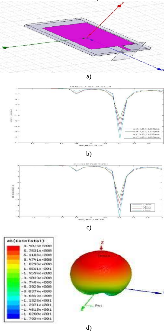
Fig 1. Rectangular patch antenna with strip line feed
