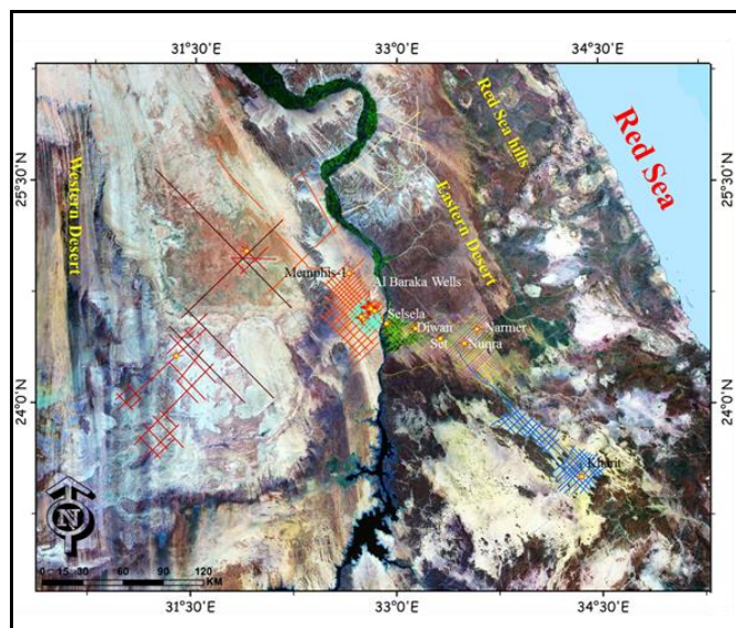
Fig. 2. Lansat image shows the location of the seismic coverages with different colors, and boreholes in the study.
