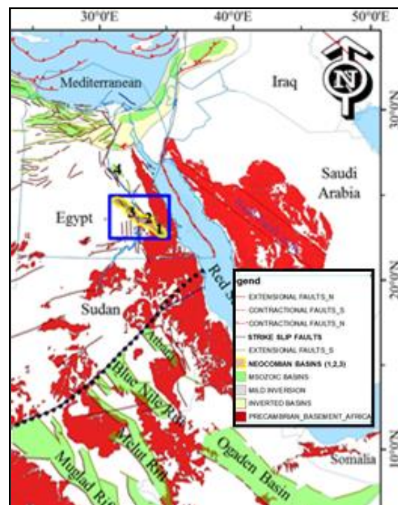
Fig. 1. Location map shows the three studied basins (1 Kharite, 2 Nuqra, 3 Komombo), and Mesozoic sedimentary basins (green color) in Egypt and Sudan (modified after Bosworth, 2008)
