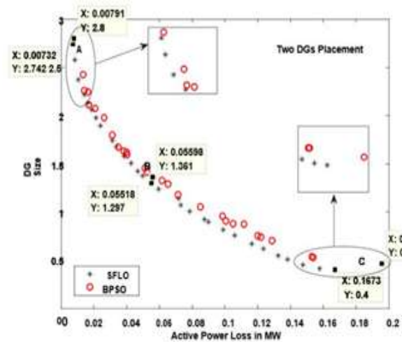
Figure 9: Comparison of Pareto-fronts of SFLO algorithm and BPSO algorithm for two DGs placement
