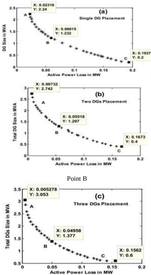
Figure 7: Pareto-front of non-dominated solutions for single, two and three DGs placement in IEEE 69-bus system of case B
