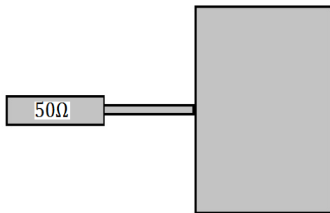
Fig. 2. Microstrip line feed [13]
