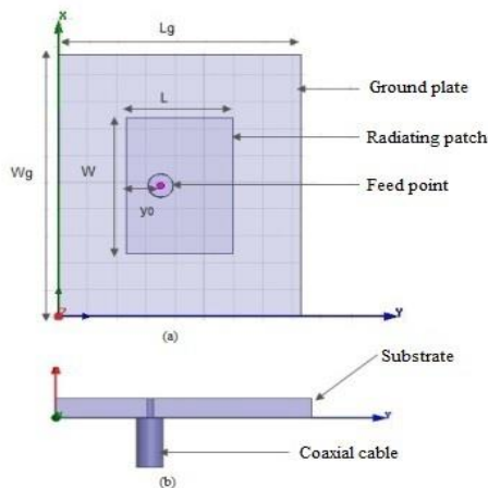
Fig. 1. Geometry of coaxial feed microstrip patch antenna [15]
