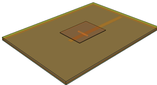
Fig. 3. Aperture Coupled Microstrip Patch Antenna, Transparent Structure: Bottom Layer: Microstrip, Center: Ground Plane & Slot, Top: Patch [11]
