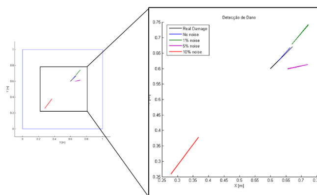
Fig. 5. Crack detection results considering random noise data.
