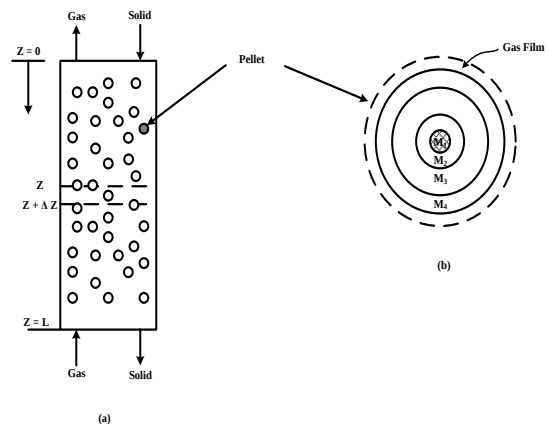
Figure 5: Moving Bed Reactor with Porous Pellets
