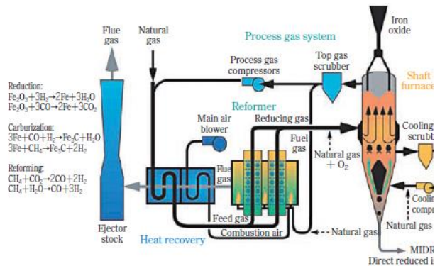
Figure 3: Midrex Direct Reduction flowsheet. Source: [6].
