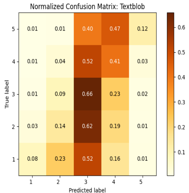
Fig 7. Confusion Matrix for Textblob
