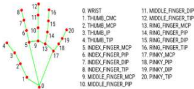
Fig. 2. 21 Hand Landmarks
