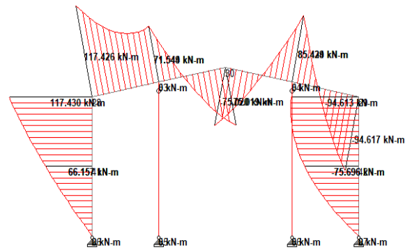
Fig 14. Gable end frame of model PEB1
