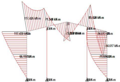
Fig 2. Bending Moment diagram along z axis for PEB1
