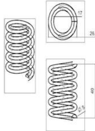
Fig.7 Spring
