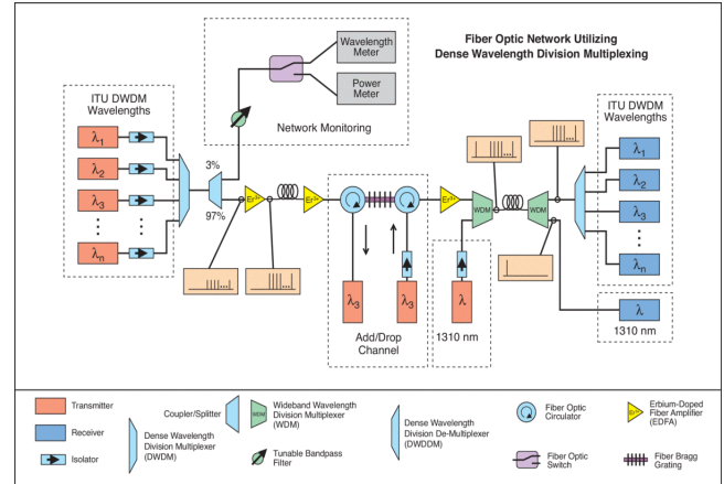
Fig.5. Optical Network Configurations [8]
