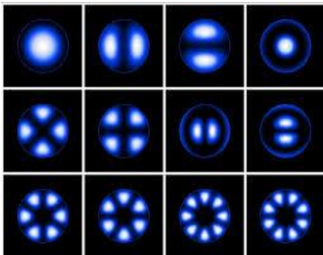
Fig.2. Optical Fiber Modes [6]
