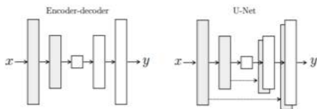
Fig 2.1 Two choices for the architecture of the generator. U-net architecture. [13]
