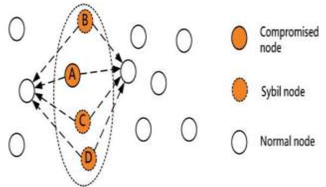
Fig.2. Sybil Attack [6]
