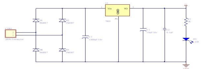
Fig. 5 Power Supply Design
