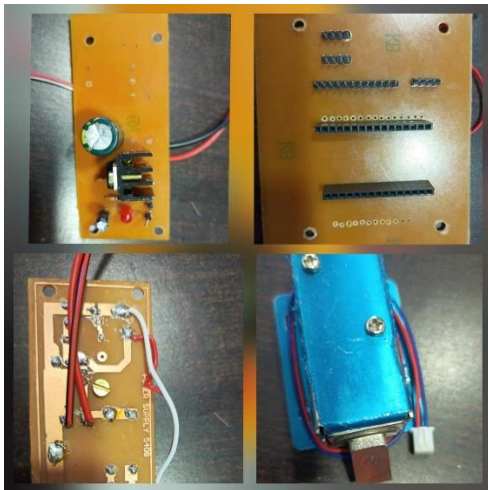
Fig. 7 Instruments Assembling
