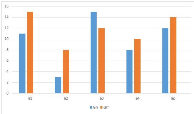
Fig. 6. Histogram for the frequency of the labels a1, a2 to ap in Graph ( G_h and G_1 )
