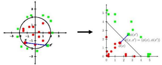
Fig. 5. Graph Kernel
