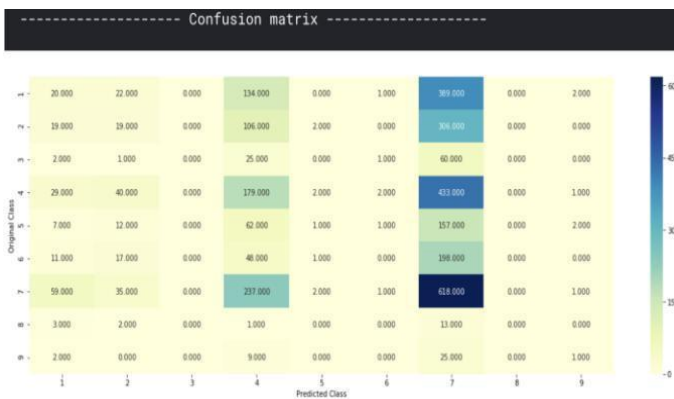
Fig no. (5) Calculating Log Loss (6) Recall matrix (7) Precision matrix (8) Confusion matrix
