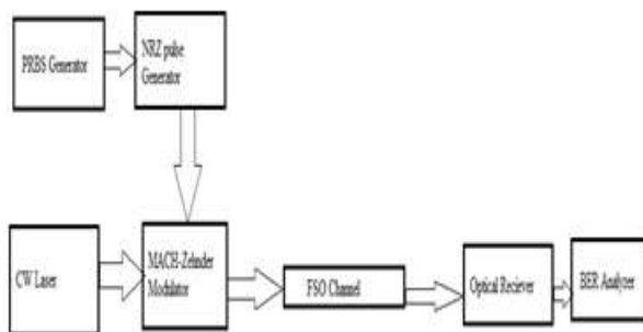
Fig. 3. Block diagram of the system model
