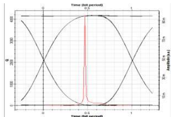
Fig i: Eye diagram at range 5m at beam divergence 0.2
