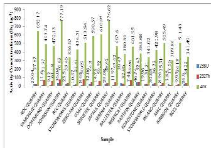
Figure 2 Activity Concentrations of Natural Radionuclides in Samples
