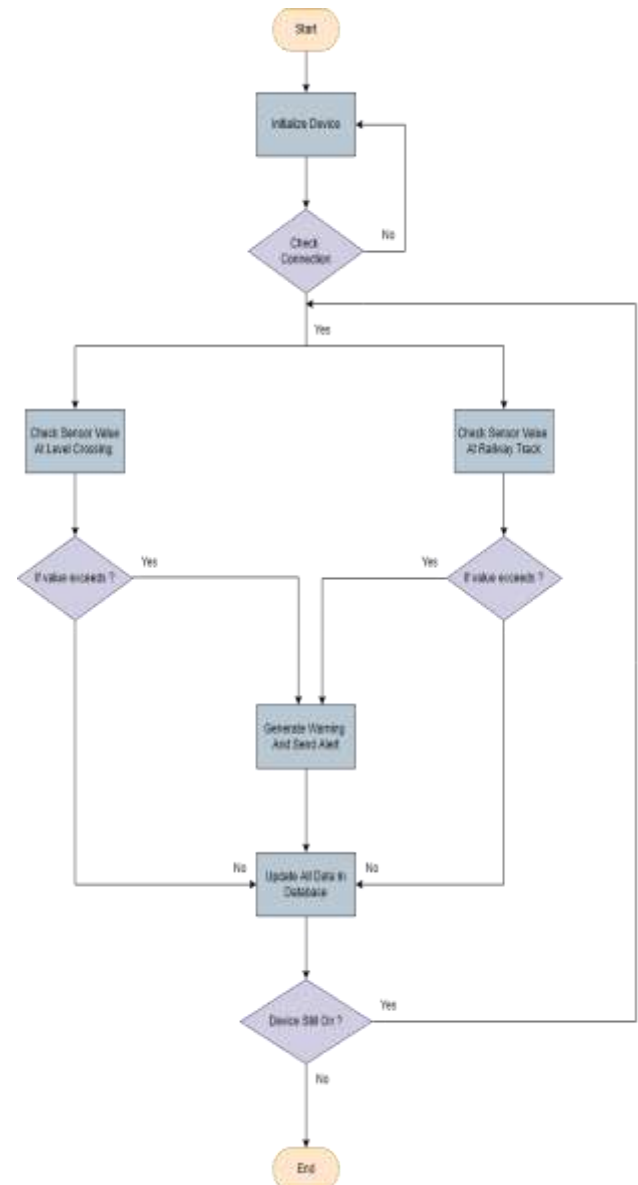
Fig. 6. Flowchart For ESP-8266
