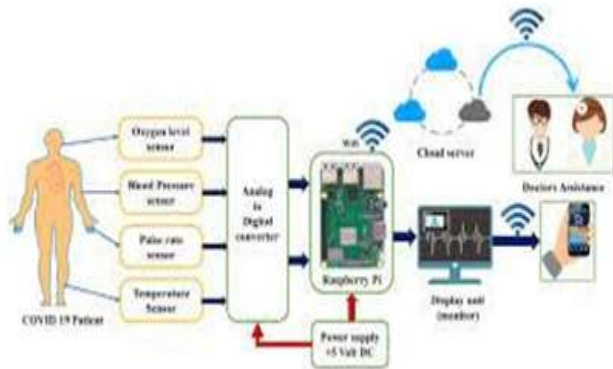
Fig 2: Proposed Architecture
