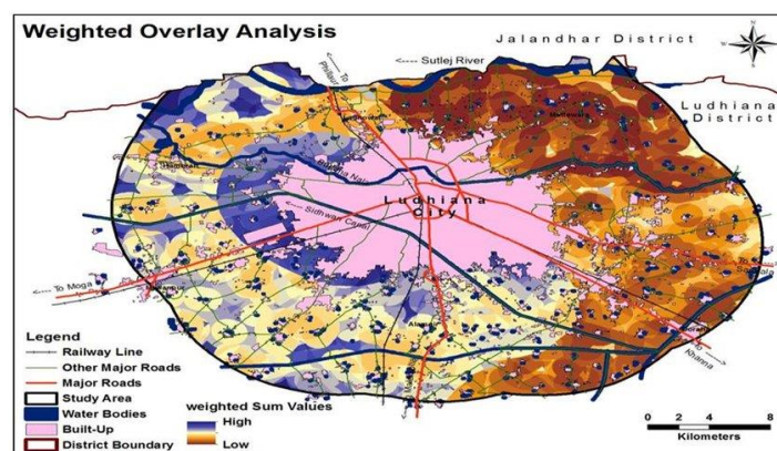
Fig 1. Weighted Sum Average of Ludhiana district Solid Waste
