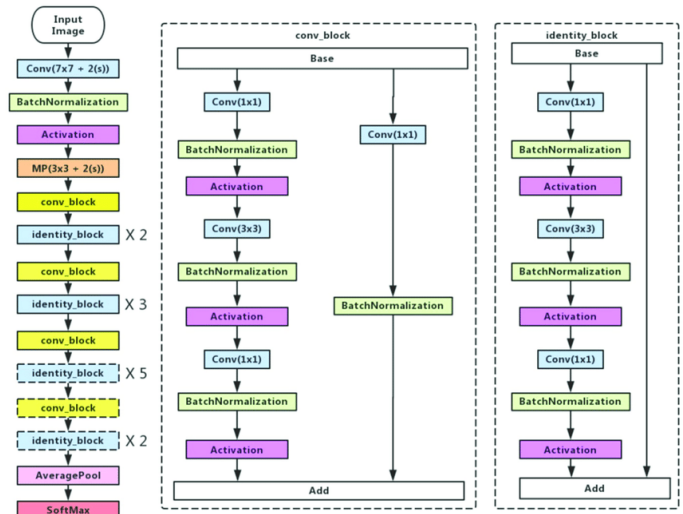
Fig 4. Architecture of ResNet50
