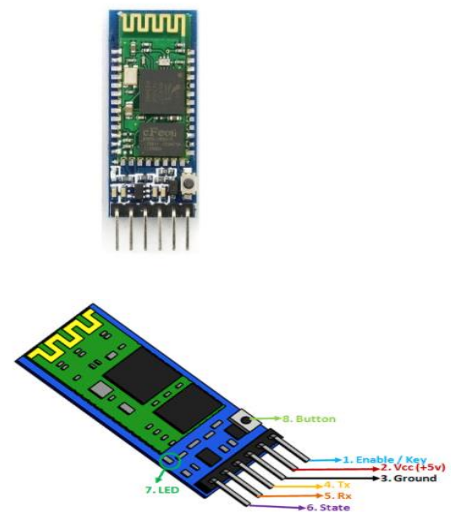
Fig 12. HC-05 Bluetooth
