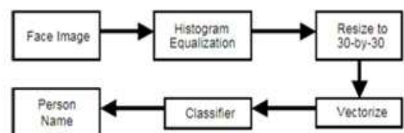
Figure 5. Algorithm for Face detection part.
