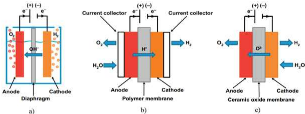
Figure 2. Schematic illustration water electrolysis cell systems, a) Alkaline electrolyzer, b) Polymer-electrolyte membrane electrolyzer, c) Solid oxides electrolyzer (Coutanceau, et al., 2018)
