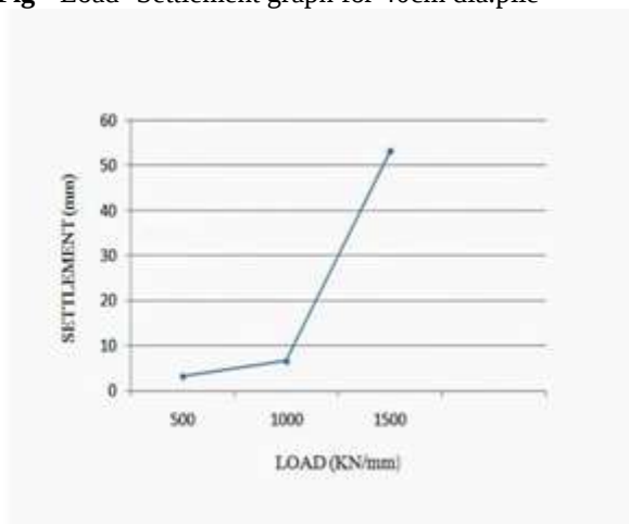
Fig - Load- Settlement graph for 50cm dia.pile
