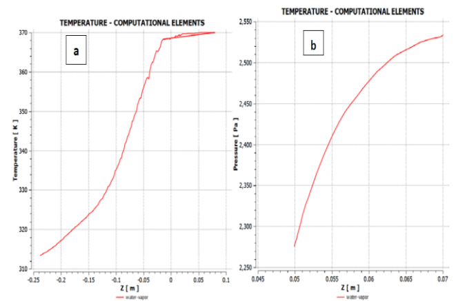
Fig. 6. (a) Temperature and (b) pressure plot of Computational Elements
