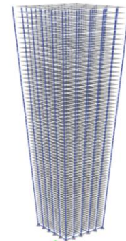
Fig. 1. (b) Analytical model provided without the outriggers
