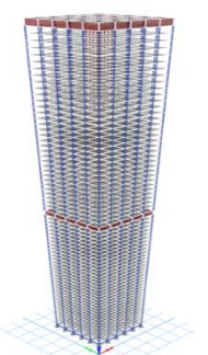
Fig. 5. Model with outriggers at H (top) and H/2
