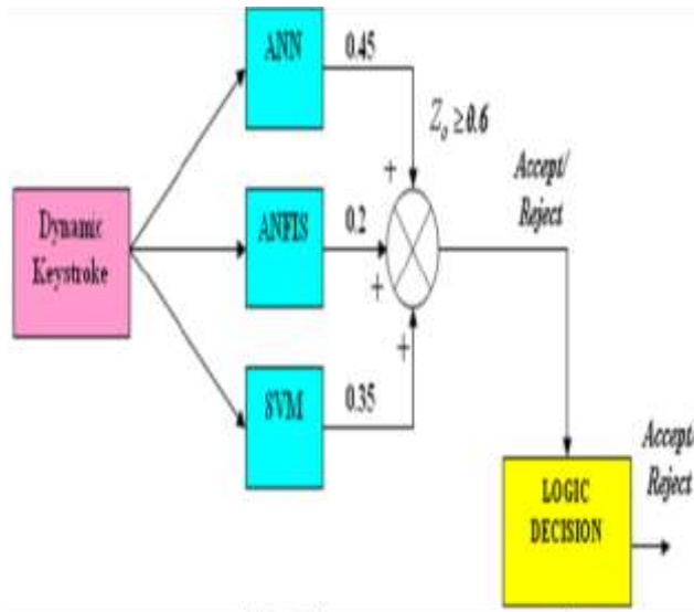
Fig. 5 Structure Chart of keystroke dynamics
