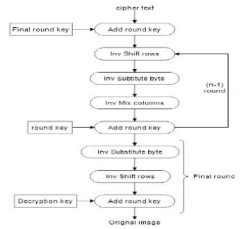
Fig2. AES Decryption
