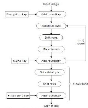
Fig1. AES Encryption
