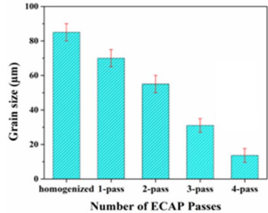
Fig. 4. Grain size in \mu\text{m} before and after ECAP process
