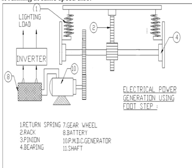
Fig. 2.3. Line Diagram for Foot Step Power Generation
