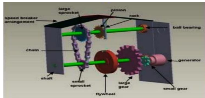
Fig. 3.2. Model of Speed Breaker Mechanism
