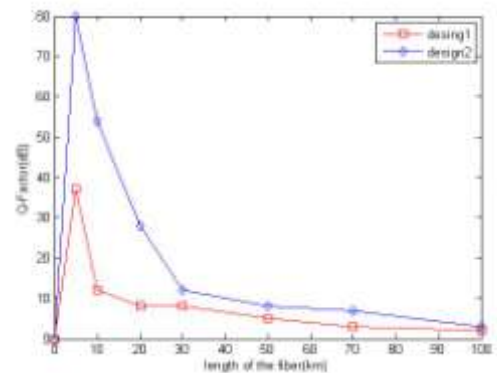
Fig.10: Graph of OFC length (km) versus Q-Factor (dB)
