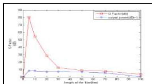
Fig.7: Graph of output power (dBm) with Q-Factor (dB) verses OFC length (km)
