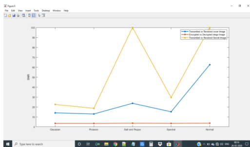
Figure 16 the Graphical Representation of the Values of SNR against the Different Types of Attacks
