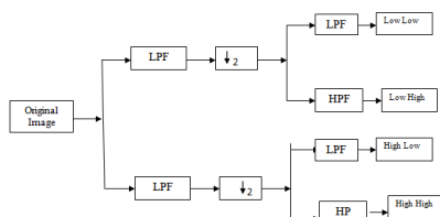
Figure 1 Dividing Images into 4 parts by applying DWT
