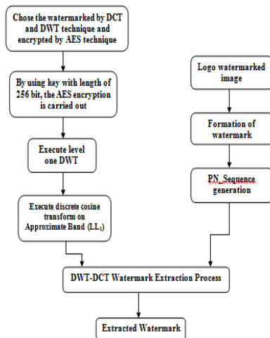
Figure 6 Extraction from Combined Discrete Wavelet and Discrete Cosine Transform and the Decryption Process for AES Encrypted Image
