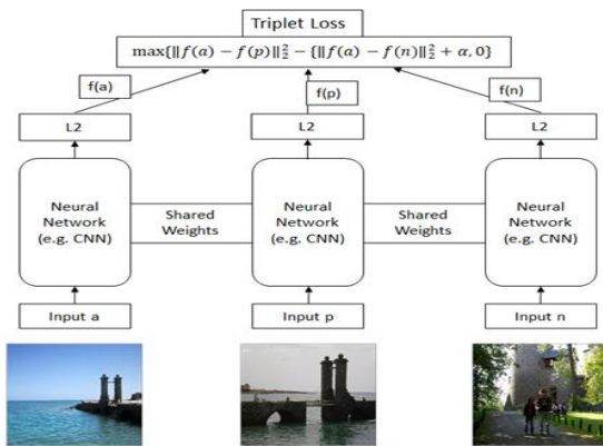
Fig. 1. Triplet Network
