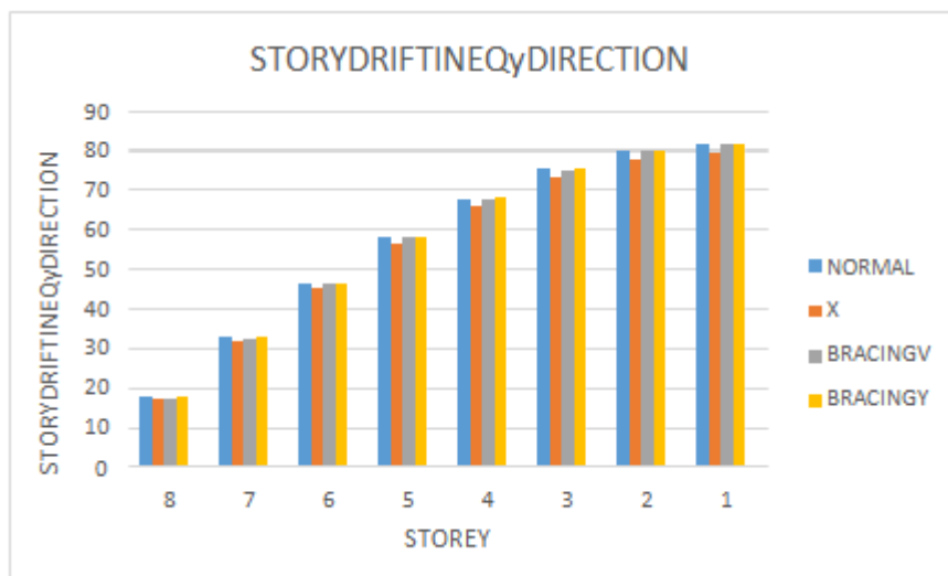
Graph 6.10 Storey Drift in EQy direction for Sand
