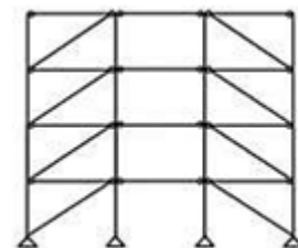
Fig 2.2 Single diagonals
