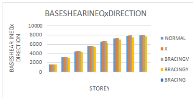
Graph 4.11 Base Shear in EQ x direction for Sand
