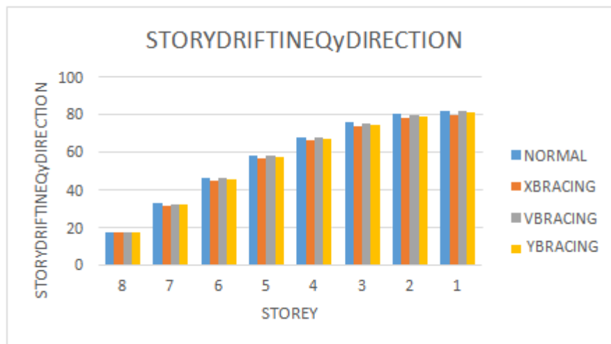
Graph 4.4 Storey Drift in EQ y Direction for Clay
