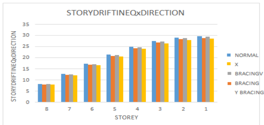
Graph 4.9 Storey Drift in EQx direction or Sand
