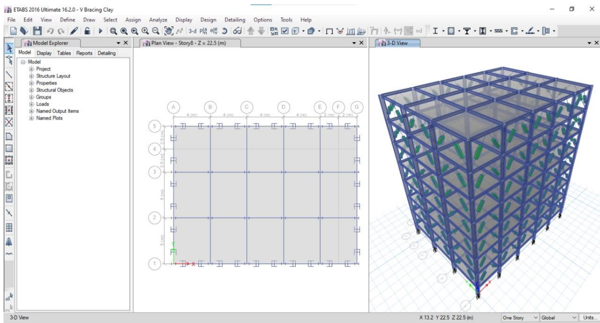
Fig 3.7: With Inverted V Bracing
