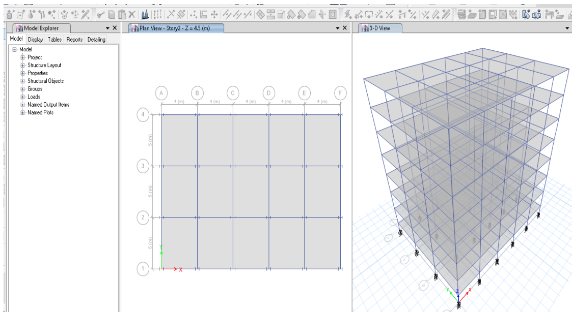
Fig 3.5: Without Bracing
