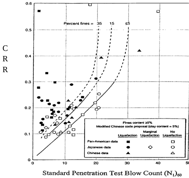
Fig6:- (N_1)_{60} vs. CRR curve
