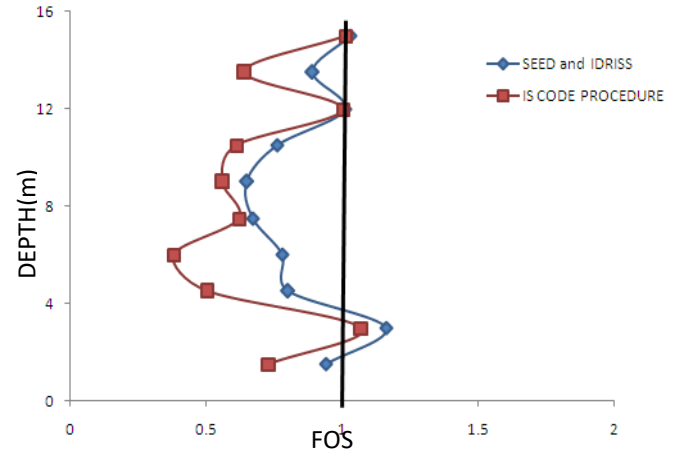
Fig 10:- FOS vs Depth
