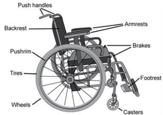
Fig.1: Components of manual wheelchairs [7]
