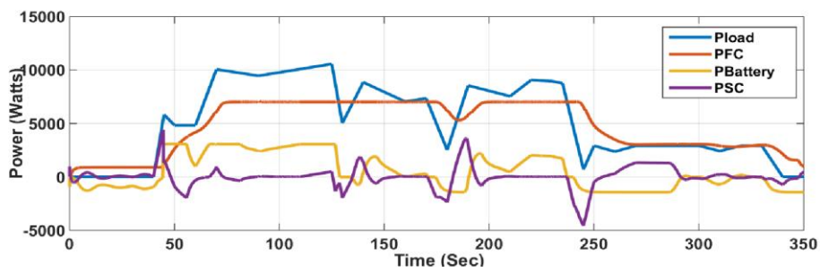
Fig. 7. Power.
