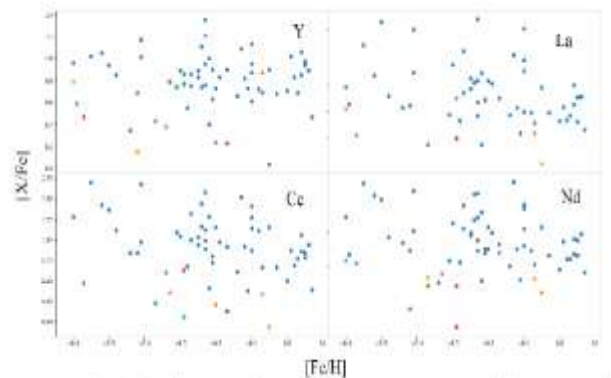
Fig 7. The Abundance ratio of the heavy elements (like Y, La, Ce, and Nd) from the programme stars are compared to [X/Fe] of the other barium stars obtained from Kuruz database.
