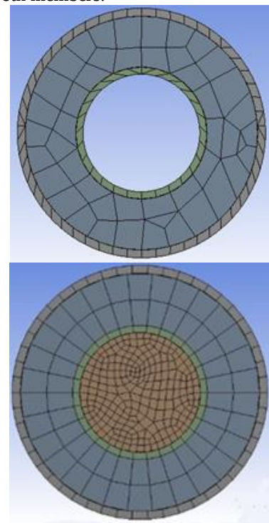
Fig. 2 Meshed view
