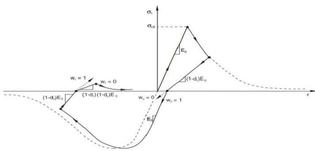
Figure 1. Concrete damaged plasticity modified stress/strain curve
