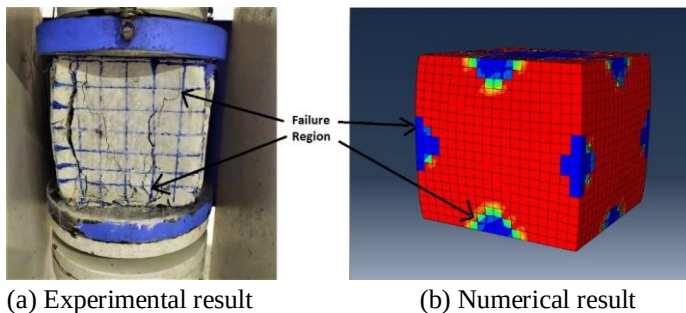
Figure 5. Comparison of failure mode for bone-China ceramic cube
