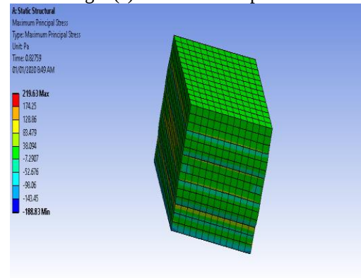
Fig 5 (b) Total deformation in a composite sample
