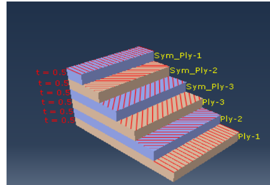
Fig 7(a) Laminate stacking sequence in a circular tube
