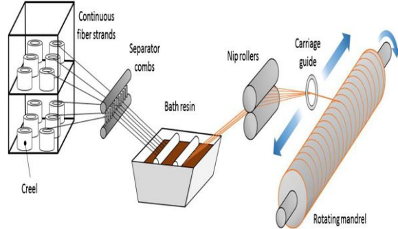
Fig. 2 Filament winging process
