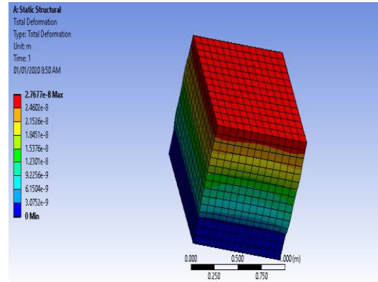
Fig 5 (a) aluminum sample
