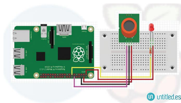
Fig 2.8.2: Connection Configuration [1]
