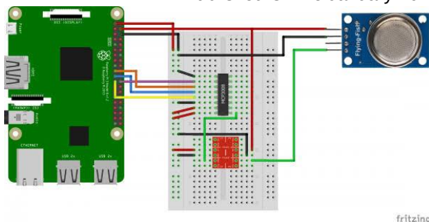
Fig 2.7.2: Connection Configuration [1]
