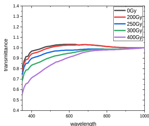
Fig. 1. Plot of Transmittance versus Wavelength for Un-irradiated (0 Gy) and Irradiated Samples of ZnSe thin films.
