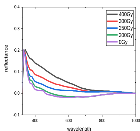
Fig. 2. Reflectance versus Wavelength for un-irradiated and irradiated samples of ZnSe thin films.
